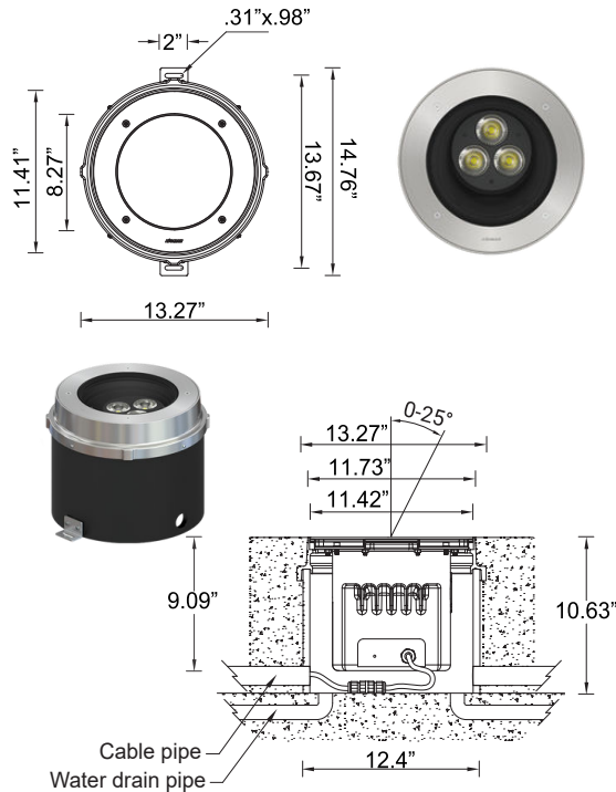
Mounting Detail
